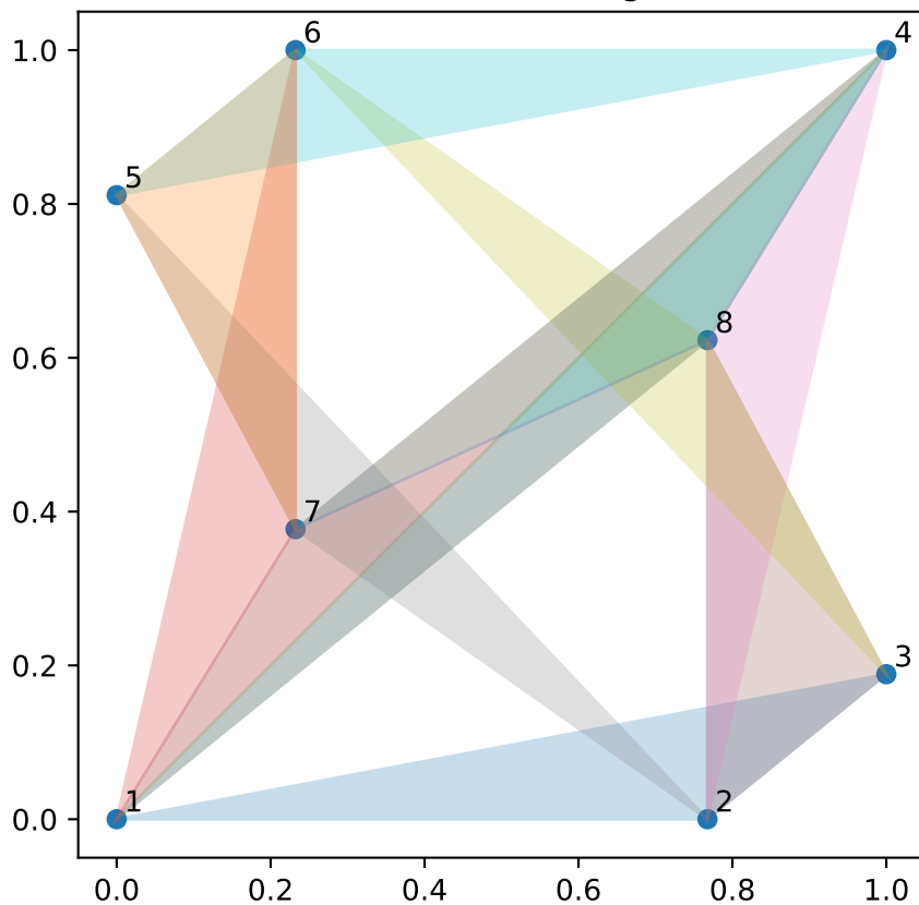
The 12 minimal area triangles for n=8
